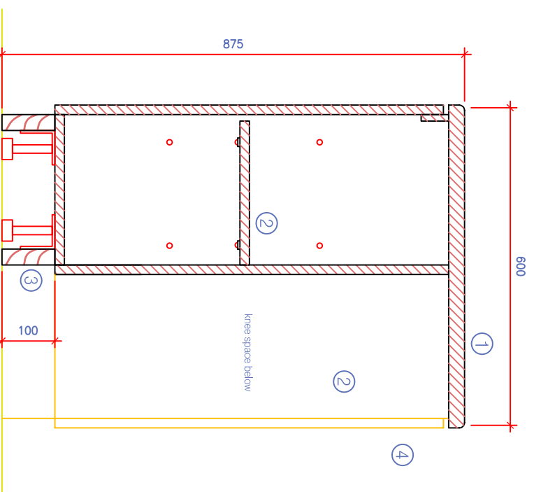
section b-b
