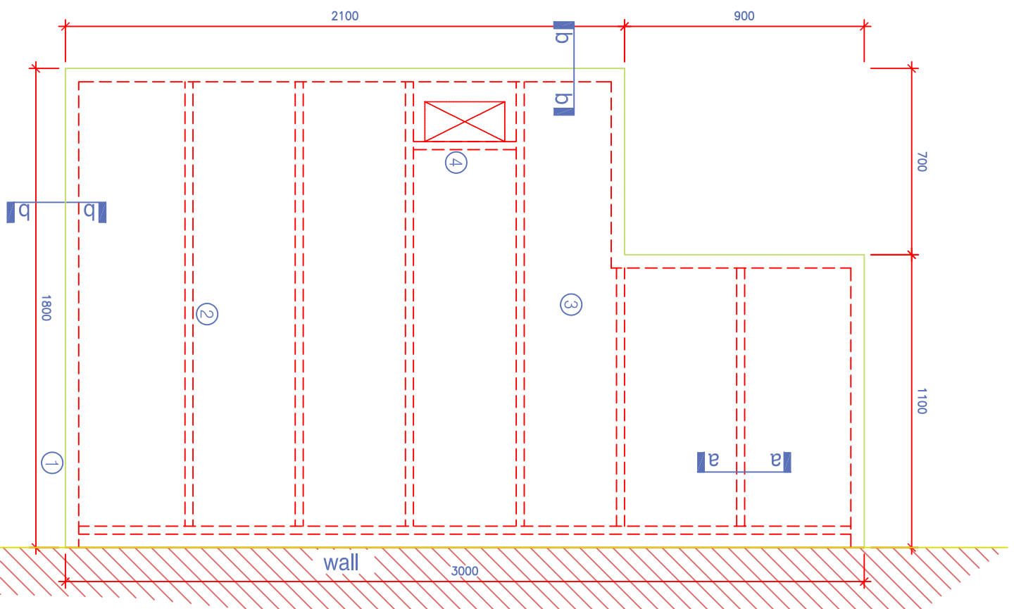
plan type 1: Science Laboratory & Demonstration Room
