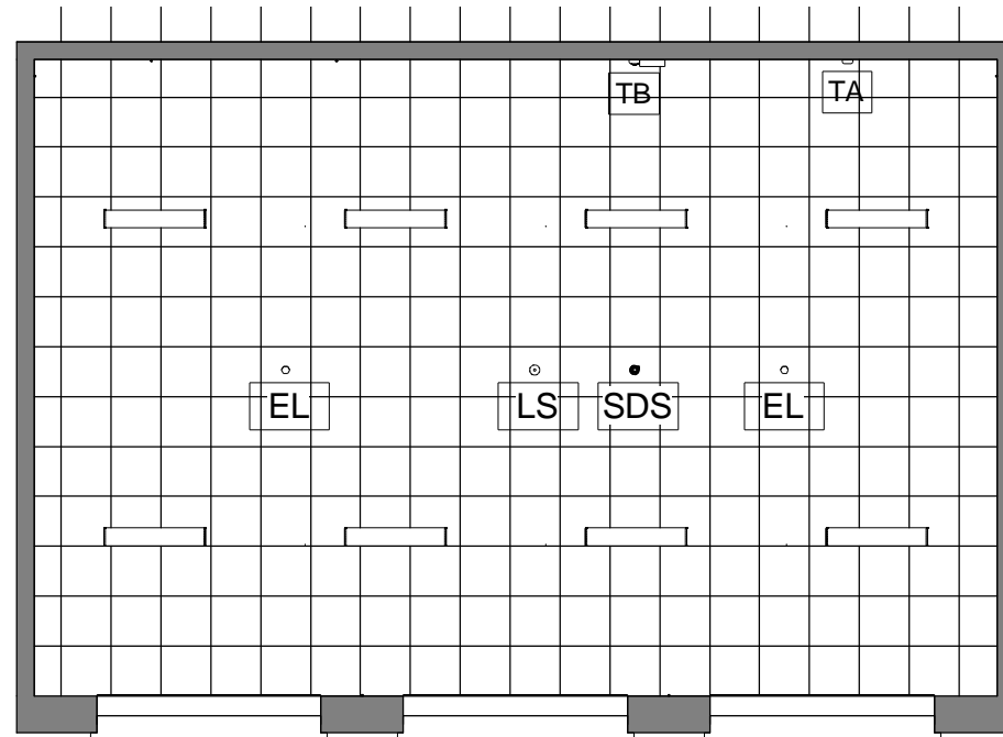
1 Indicative Ceiling Plan 1 : 100 / 500 lux
