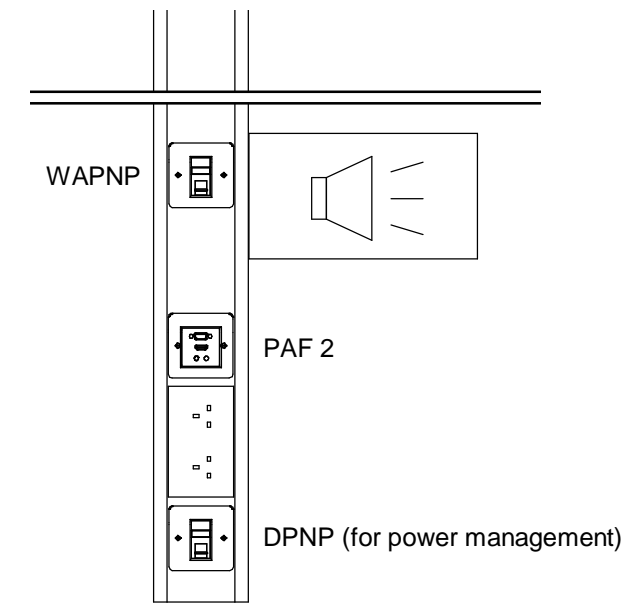
3 TB - Trunking "B" 1 : 10
