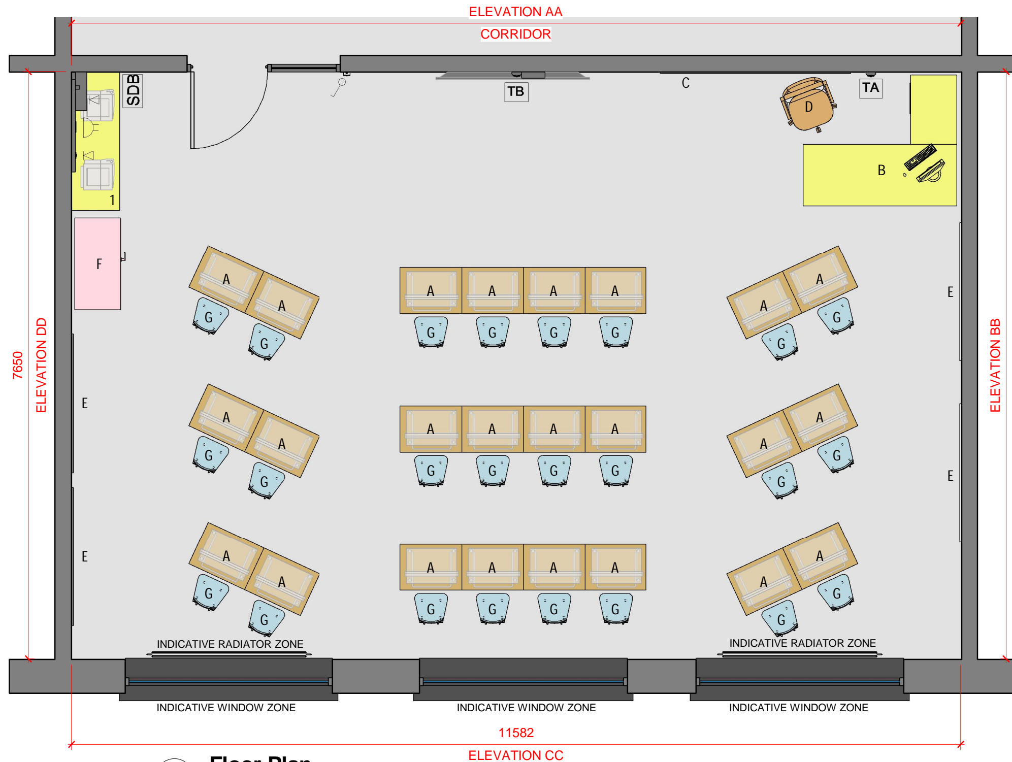
1 Floor Plan 1 : 50 / 88.60 sq.m
