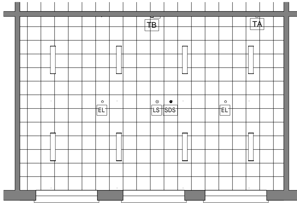
1 Indicative Ceiling Plan 1 : 100 / 500 lux
